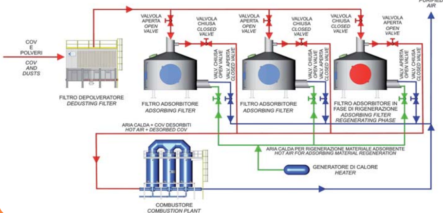
Abbattimento polveri e ammina da reparto animisteria COLD-BOX Dusts and amines treatment from COLD-BOX core-shop department
